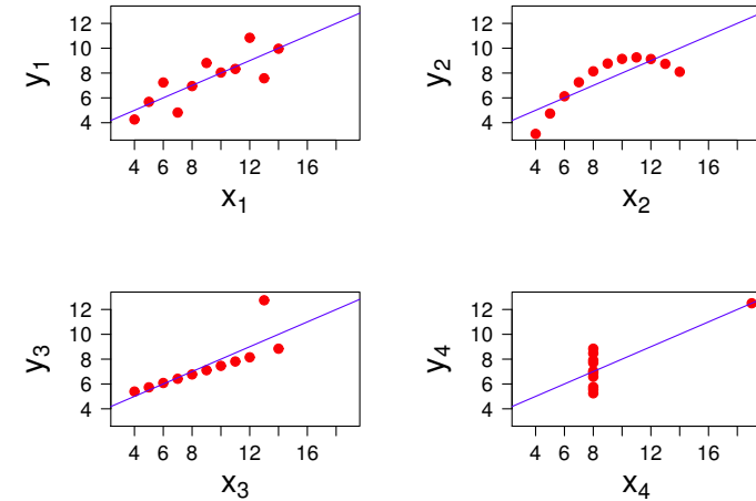
Figure 10: Anscombe's Quartet.
